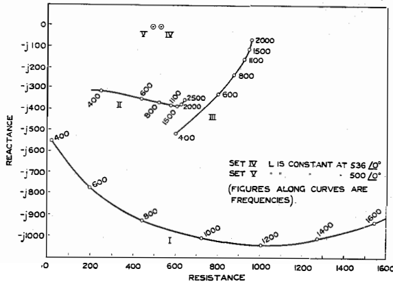
Figure 6—No-Side Tone Line Impedance for Sets Tested.
