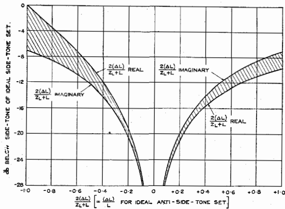
Figure 1—Side Tone of Anti-Side Tone Set.
