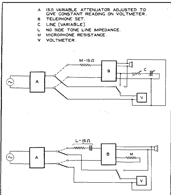
Figure 4—Measurement of Line Voltage V_L and Side Tone Voltage V_{ST} (Upper Schematic). Measurement of Received Voltage V_R from Line (Lower Schematic).
