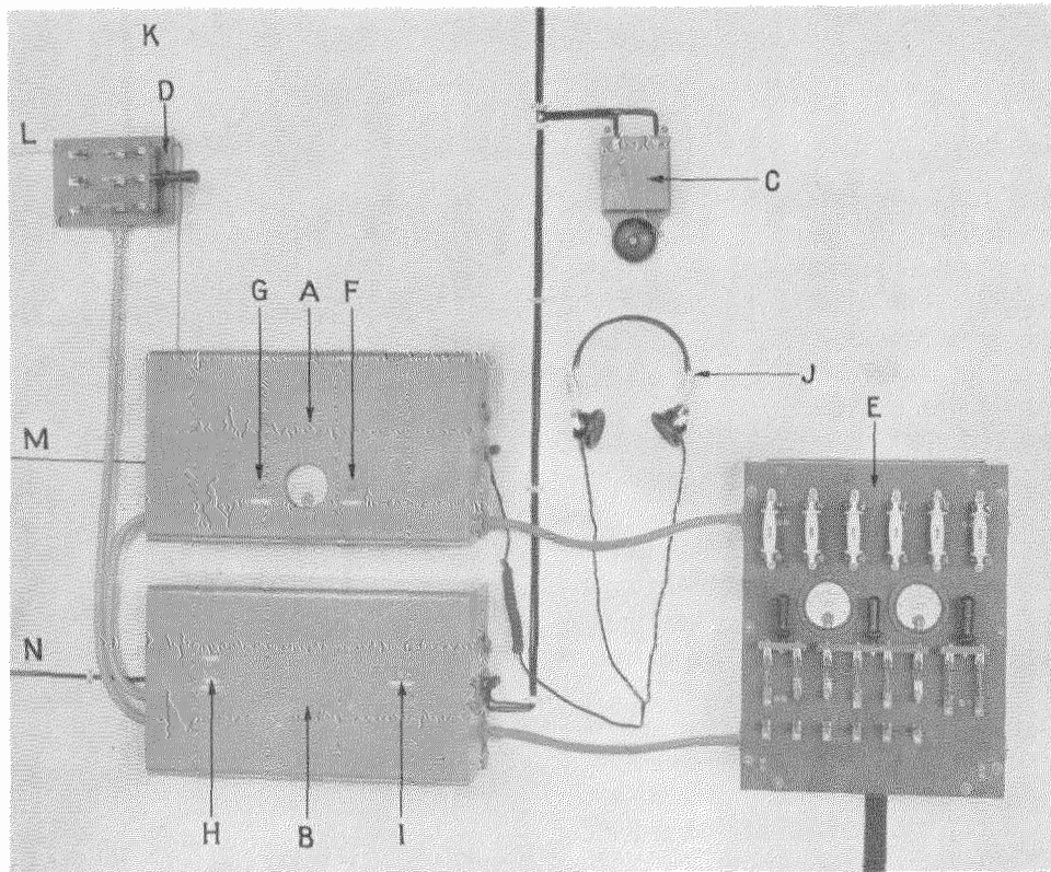
Figure 1—A.A.2.B. Auto-Alarm Assembly:
