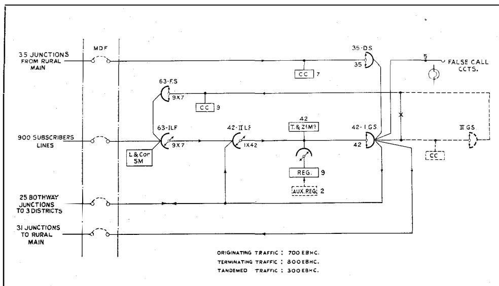
Fig. 19—Junction Diagram—Arlesheim 900 Line Centre Exchange—Basle Rural Area—Switzerland. (See Fig. 28).
