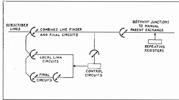
Fig. 34—Typical Diagram for District Exchange Exceeding 100 Lines.
