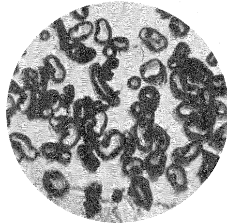
Figure 17—Cross-Section of Another "Immunised" Cotton Showing Heterogeneous Constitution of Fibre. (Magnification of this figure approximately of the order of 600).
