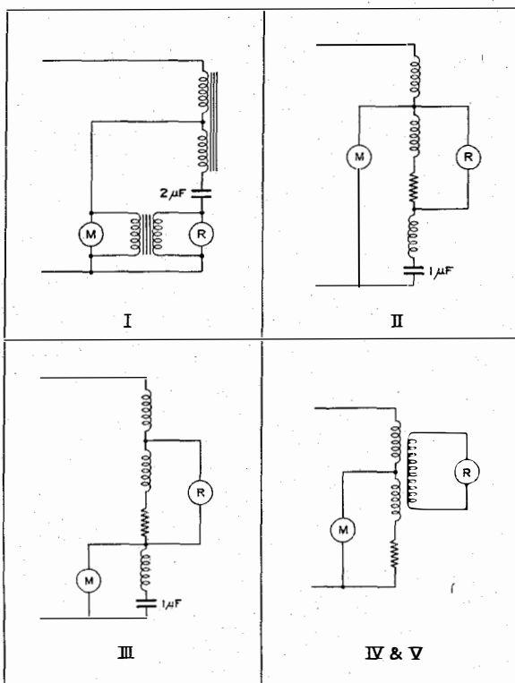
Figure 3—Schematic Circuits of the Telephone Sets Tested.
